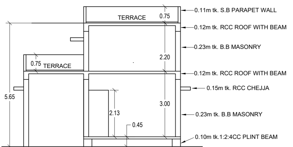
CROSS SECTION AT A-A
