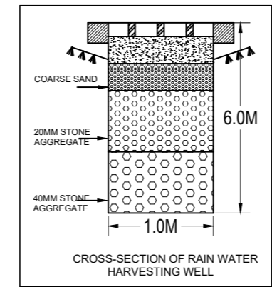
CROSS-SECTION OF RAIN WATER HARVESTING WELL
